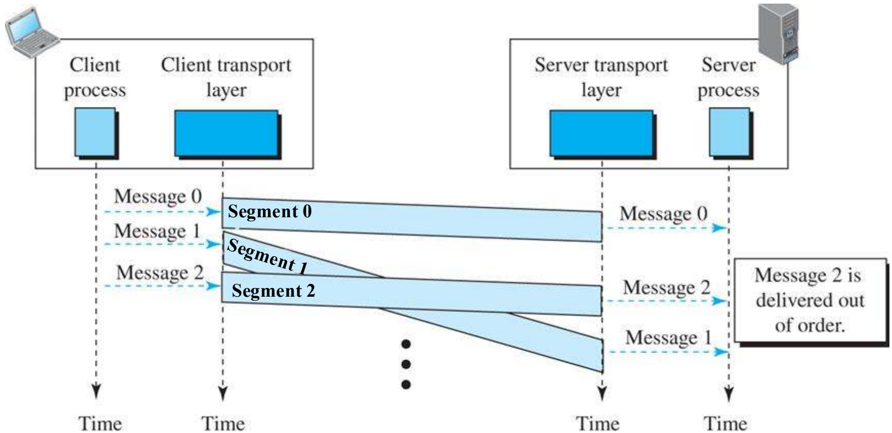
Figure 9.14 Connectionless service
